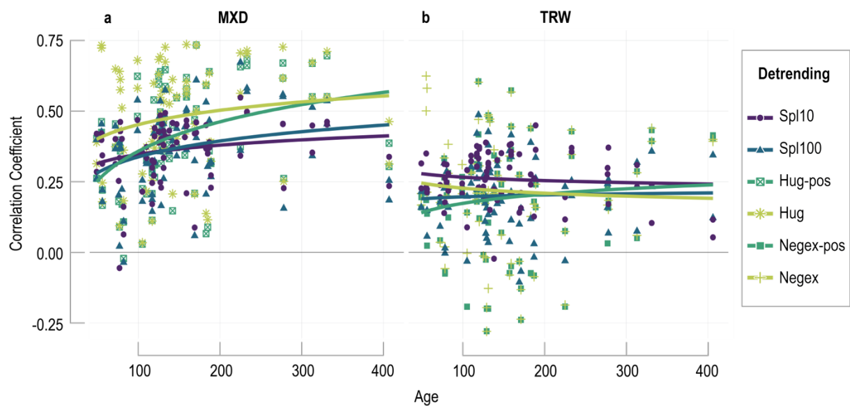
Fig. S2 Effects of the detrending on CSAE. Each dot represents a single series, each color a detrending. Bold lines are logarithmic regressions for (a) MXD and (b) TRW
