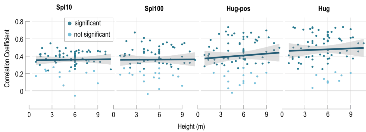
Fig. S3 MXD MJ&AS signals plotted against tree height considering different detrending
