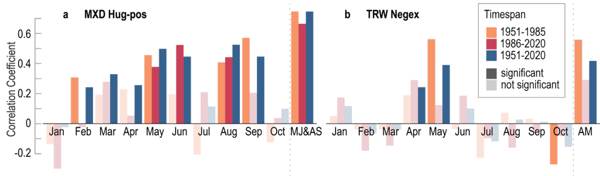
Fig. S1 Stability of the temperature signal. Three independently calibrated time periods were used to control the stability for (a) MXD and (b) TRW
