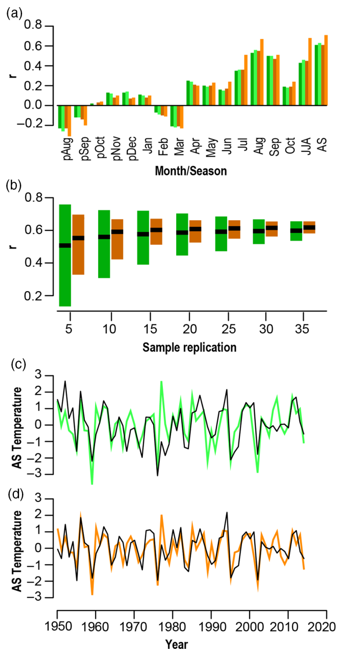
FIGURE 3 Calibration tests. (a) Pearson correlation of the 100SP (dark green), and 10SP (dark orange) chronology with temperature data from the EOBS v.15 grid 40.25°N and 20.75°E for the period 1950–2014 and respective high-pass filtered versions (light green and light orange). (b) Multiple correlation coefficients returned from calibrating a total of 2,000 100SP (dark green) and 10SP (dark orange) chronologies against August–September temperatures for the period 1950–2014. The 100SP and 10SP chronologies were established randomly selecting from 5 to 35 MXD series from a population of 43 living tree-ring series that span the full calibration period, (c) instrumental 100-year high-pass filtered August–September temperatures (black) and 100SP reconstructed temperatures (light green) and (d) instrumental 10-year high-pass filtered August–September temperatures (black) and 10SP reconstructed temperatures (light orange) [Colour figure can be viewed at wileyonlinelibrary.com ]
