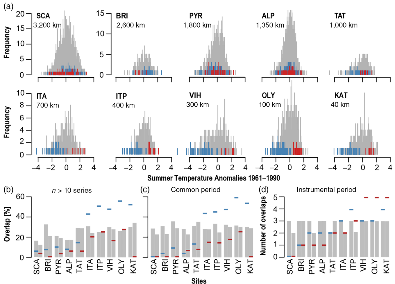
FIGURE 6 Comparison of temperature anomalies and extremes ( \pm 1.5 SD ) across Europe. (a) MXD based 100SP and 10SP temperature reconstructions from Scandinavia (SCA), United Kingdom (BRI), Spain (PYR), Switzerland (ALP), Slovakia (TAT), Italy (ITA and ITP), Bulgaria (VIH), and Greece (OLY and KAT) displayed as histograms (grey). Blue and red ticks indicate cold or warm extremes in the SMO 100SP and 10SP reconstructions and (b) percent of common cold (blue) and (warm) temperature extremes between SMO and the reconstructions displayed in Figure 6 (a) over the individual period of overlap ( n > series) and (c) the common period 1769–1978. Values refer to the mean overlap from the 100SP and 10SP reconstruction. Grey bars display uncertainty estimates derived from a Monte Carlo simulation with 1,000 randomized reconstructions. (d) Analysis was repeated comparing the overlap of the 5 coldest and 5 warmest instrumental 10-year high-pass filtered August temperatures from the EOBS v.15 grids that were used for calibration over the period 1950–2014 [Colour figure can be viewed at wileyonlinelibrary.com ]
