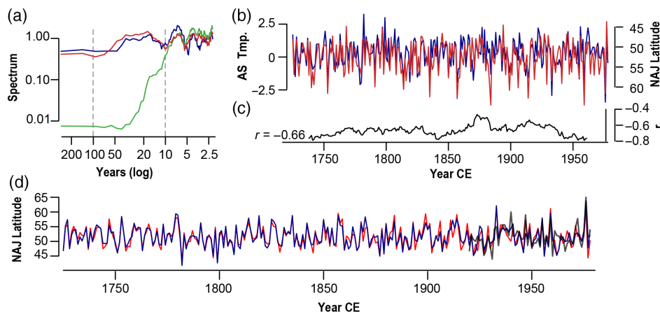
FIGURE 7 (a) Frequency analysis of the SMO 100SP (red), 10SP (green) spline August–September temperature reconstruction and reconstruction of the position of the summer North Atlantic jet (NAJ_T, Trouet et al. , 2018) (blue) over the common period 1725–1978. (b) Reconstructed 100SP August–September temperature anomalies (red), summer NAJ_T reconstruction (blue) and (c) corresponding 31-year moving window correlations (black). (d) NAJ_T (blue) and NAJ_K (red), a reanalysis of the latitudinal jet stream position using the SMO tree-ring data instead of the original NEMED compilation and instrumental August NAJ position (black) [Colour figure can be viewed at wileyonlinelibrary.com ]
