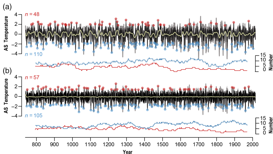
FIGURE 5 Northeastern Mediterranean annually resolved August–September temperatures back to 738 CE and cold (blue) and warm (red) temperature extremes that exceed the threshold of \pm 1.5 SD and corresponding number of extremes in running 100-year windows (lower panels). Panel (a) shows an August–September temperature reconstruction and extremes derived from a 100SP standardized chronology (black), the 15-year smoothed version (yellow) and uncertainty estimates based on the sample bootstrap error (grey) and (b) same for a 10SP chronology [Colour figure can be viewed at wileyonlinelibrary.com ]
